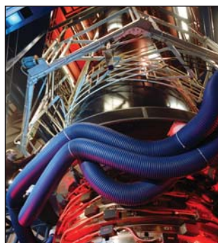
NEW 3-LAYER CO-EXTRUSION LINE 25 foot wide seamless geomembranes, accordion folded for ease of shipping and handling.
